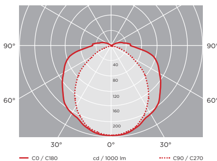
Retrofit LED 771-Pro LT, (1x1200mm), 1x14,5W (LED tube)
