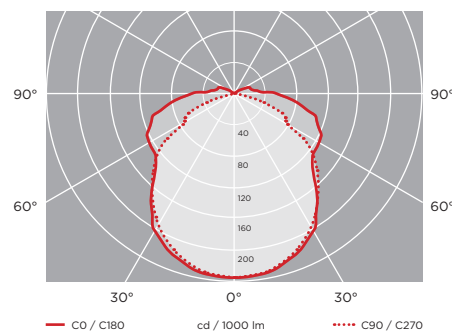
Retrofit LED 771-Pro LT, (2x1500mm), 2x20W (LED tube)
