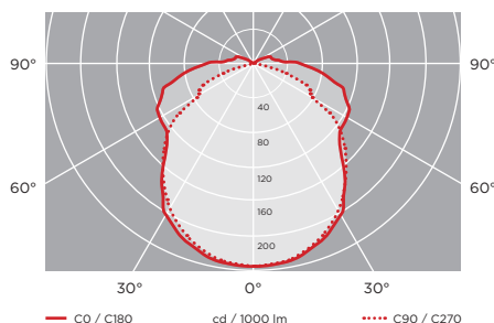
Retrofit LED 746-Pro LT 2x1500mm 2x20W (LED tube)
